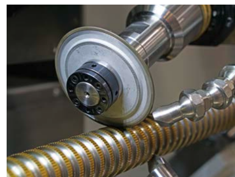
Sharpening process
